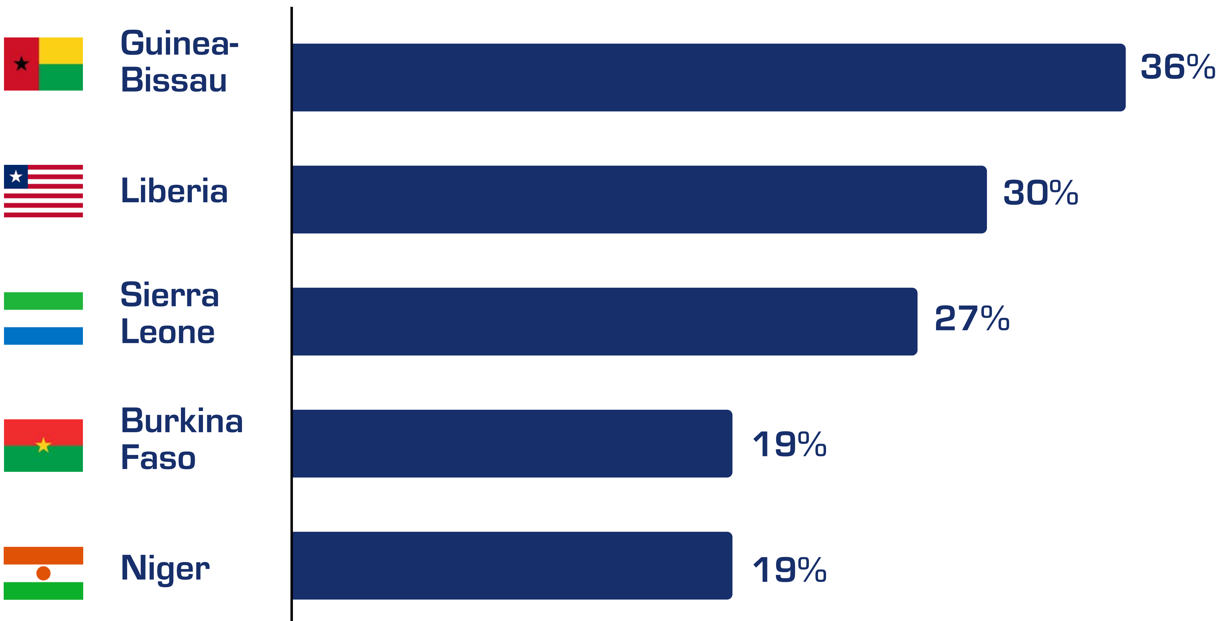
Electrification rate [%] – 2023
