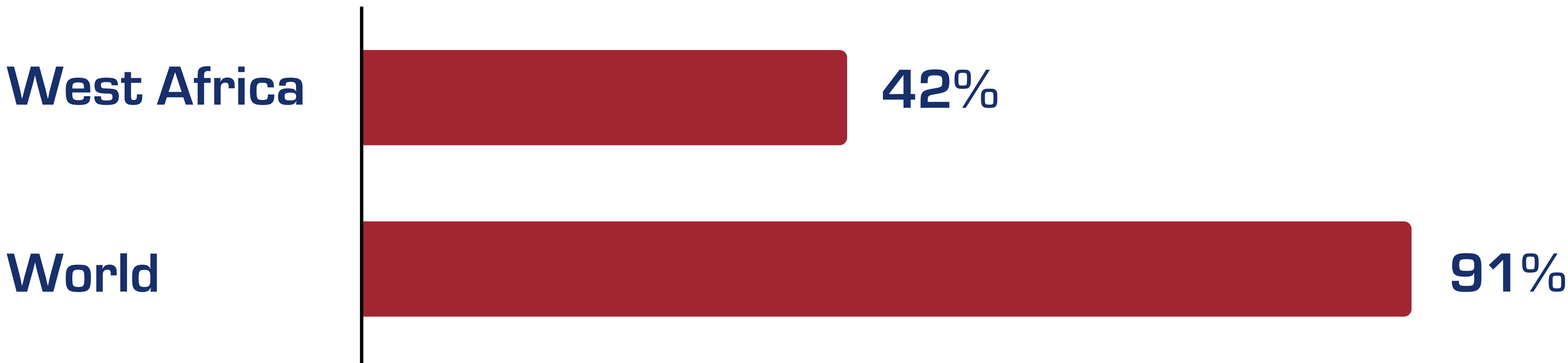
Electrification rate [%] – 2023
